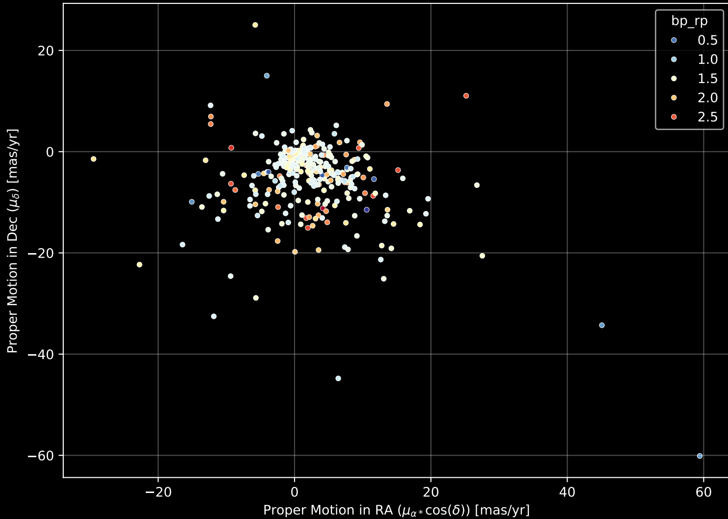
APOGEE DR17 Field: [155-27_btx] Proper Motion Diagram (n= 322)
