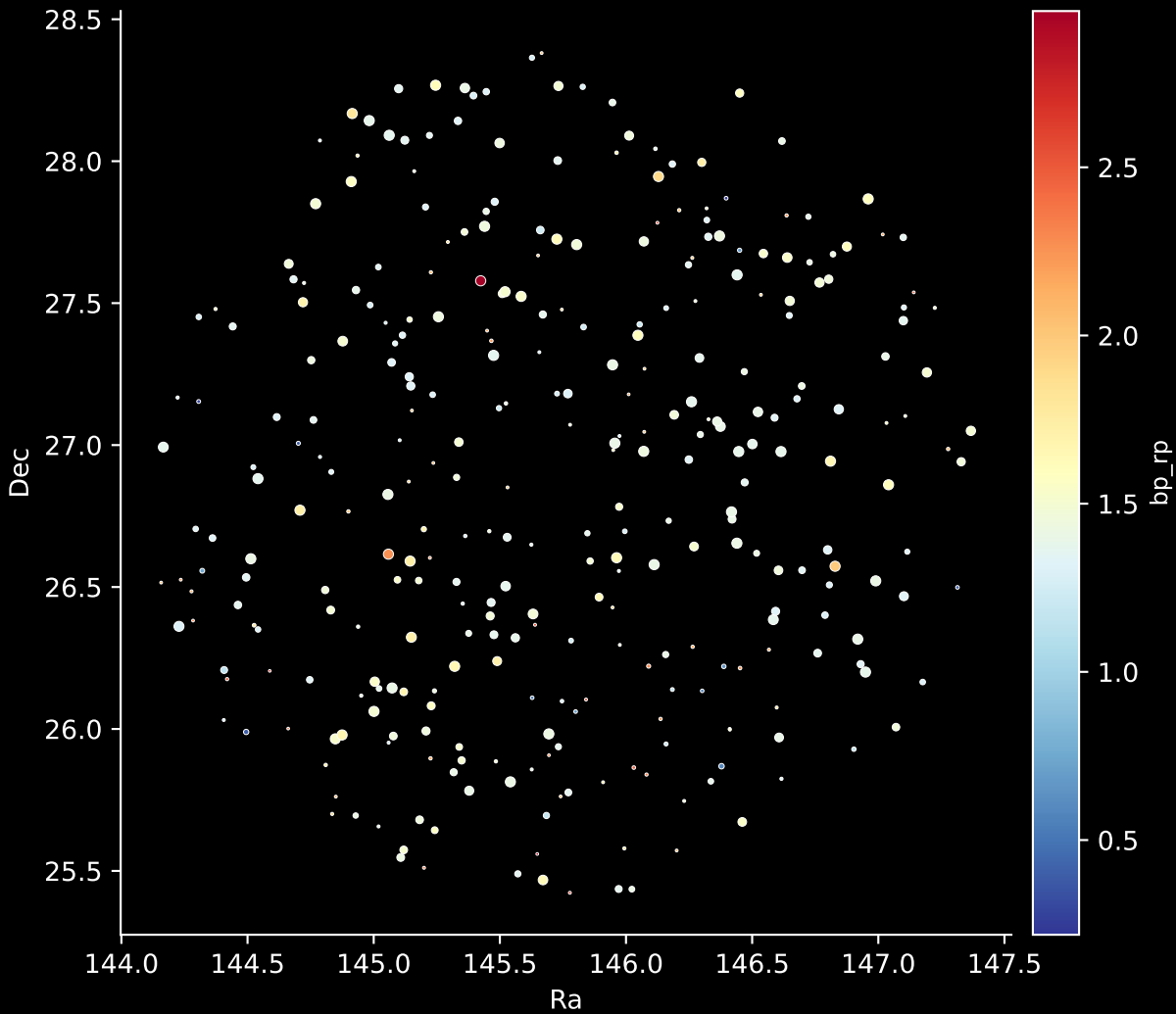
APOGEE DR17 Field: [155-27_btx] Stars: 322
