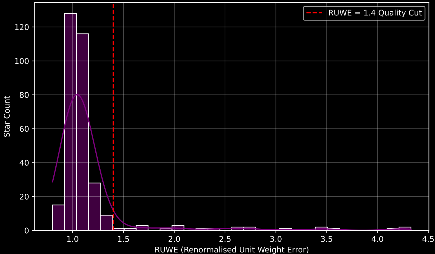
GAPOGEE DR17 Field [155-27_btx] RUWE Distribution (n= 318)
