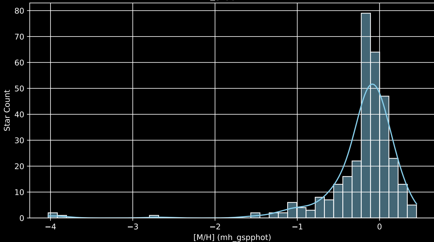
APOGEE DR17 Field: [155-27_btx [M/H] (mh_gspphot) (n= 320)
