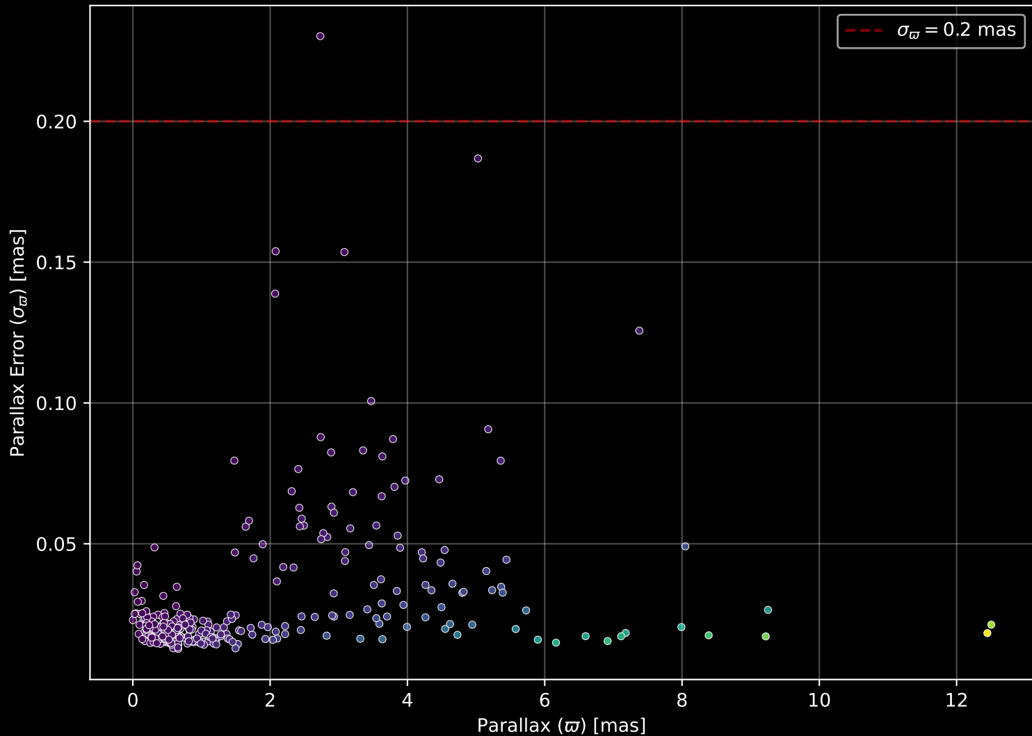
APOGEE DR17 Field: [155-27_btx] Parallax Quality (n= 322)
