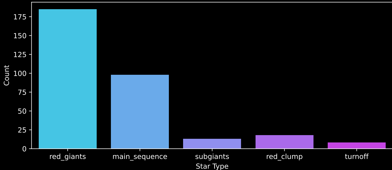
APOGEE DR17 Field: [155-27_btx] Count plot of Star Type
