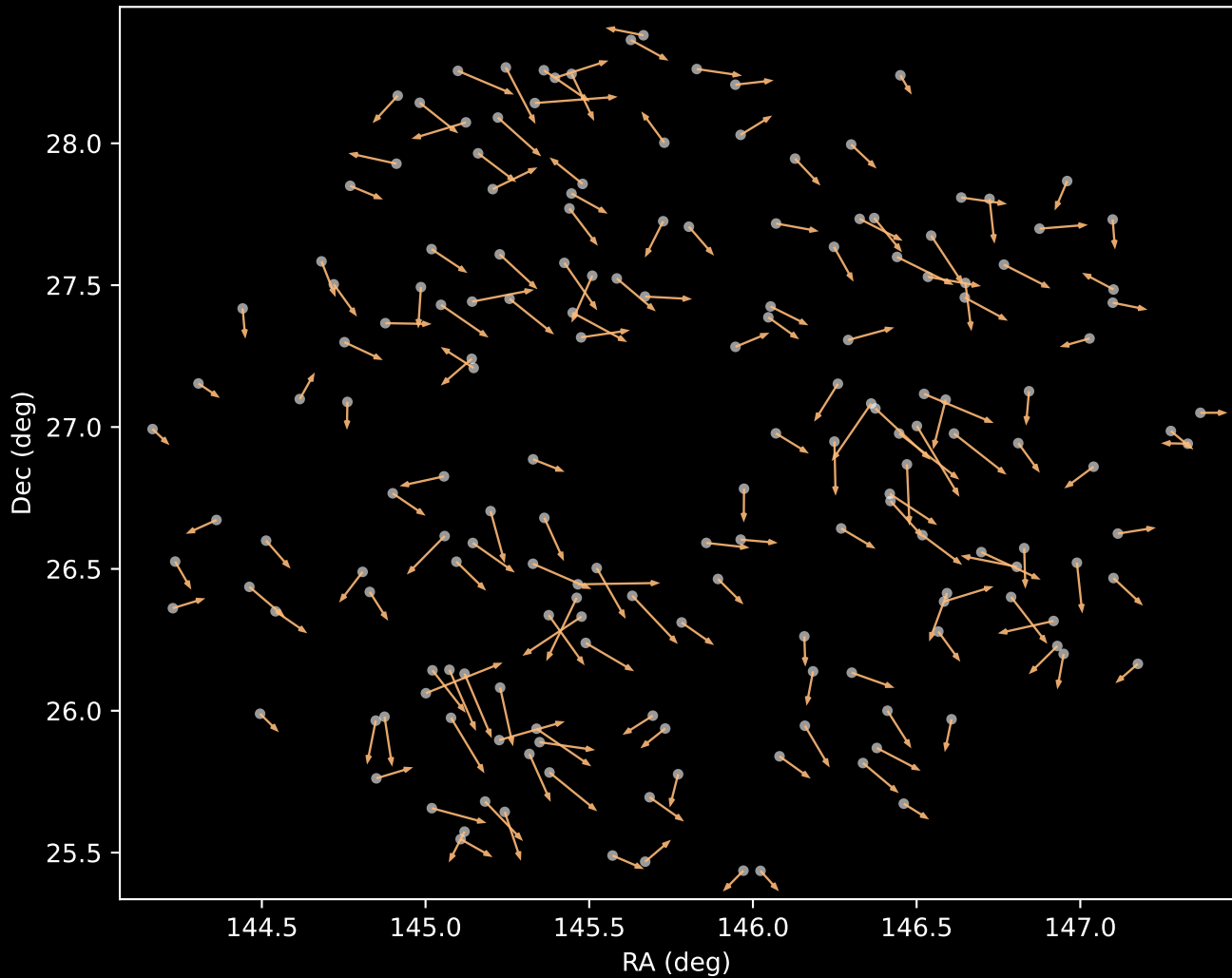
APOGEE DR17 Cluster 3 Proper Motion Vectors (n=175)
